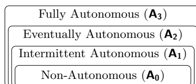
Fig. 1: Taxonomy levels.
